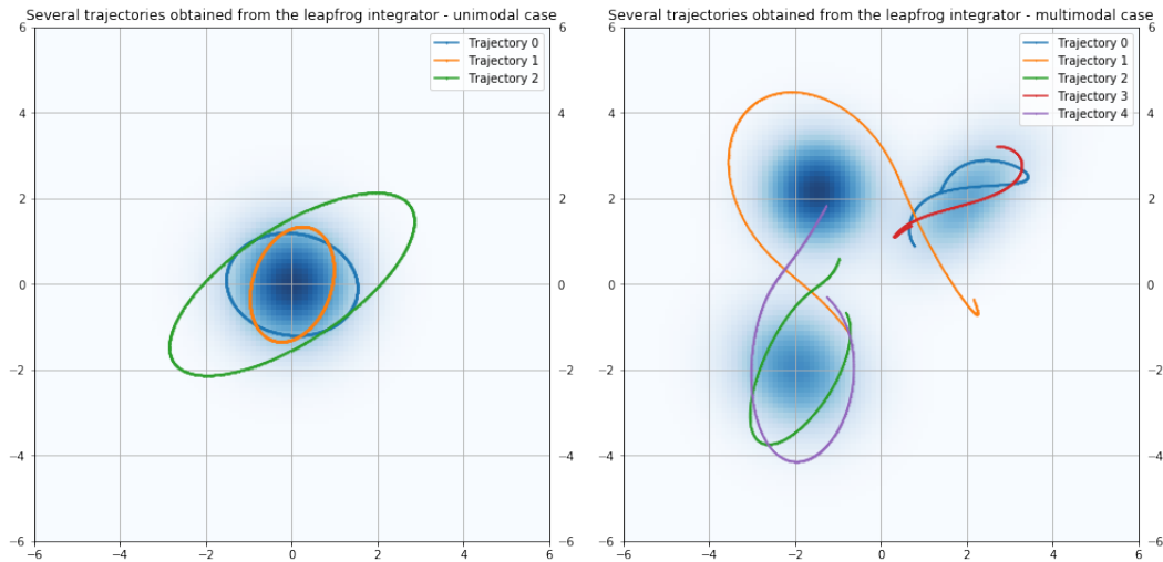
Figure 7.1.1 displays several trajectories of a HMC sampler with leapfrog integrators with various lengths when the target density a mixture of Gaussian distributions. This figure highlights the fact that the proposed moves provided by the leapfrog integrator allow to explore widely the space and to jump from a mode to another.
